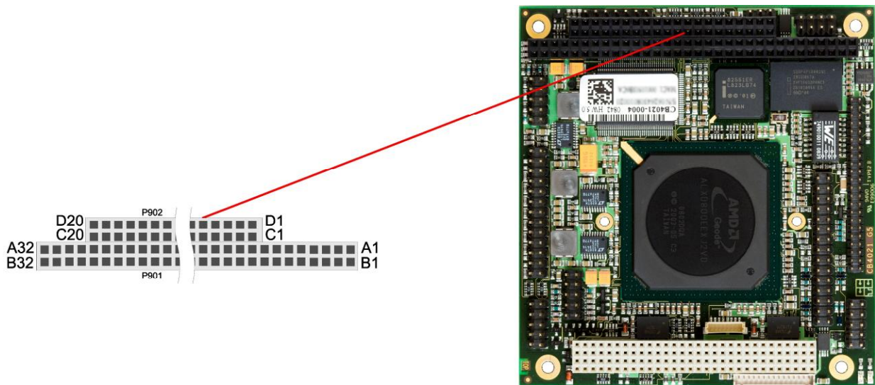
Pinning of the standard 8 bit PC/104 connector.
