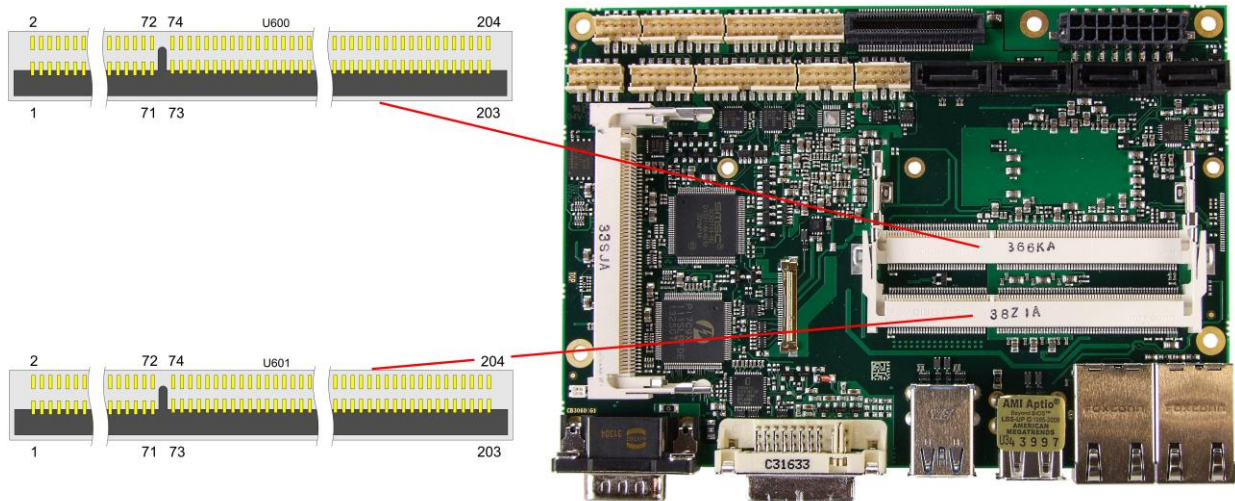
Pinout SO-DIMM204:
