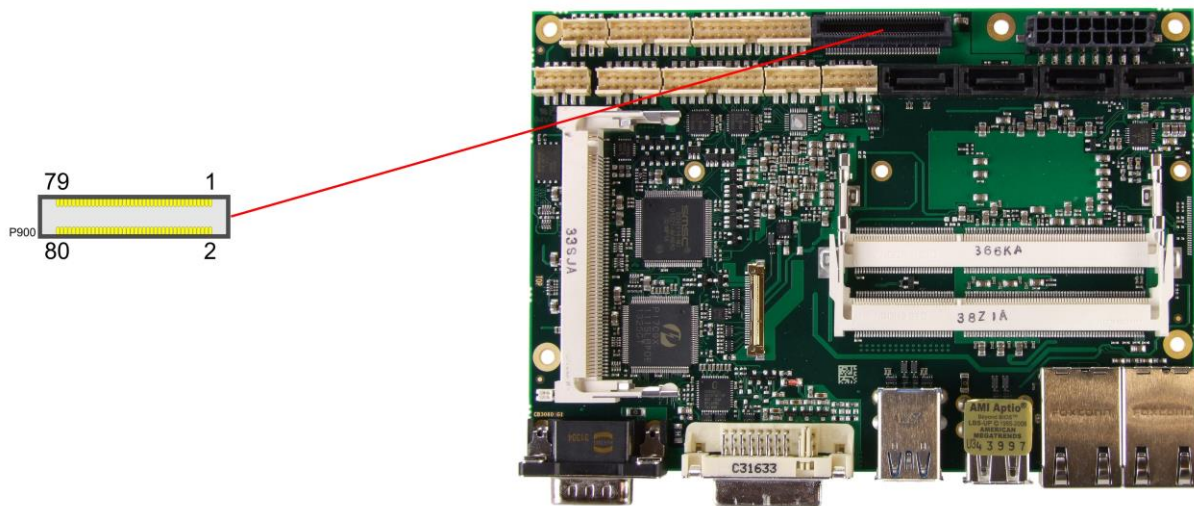
Pinout 2x40 pin connector PCIe:
